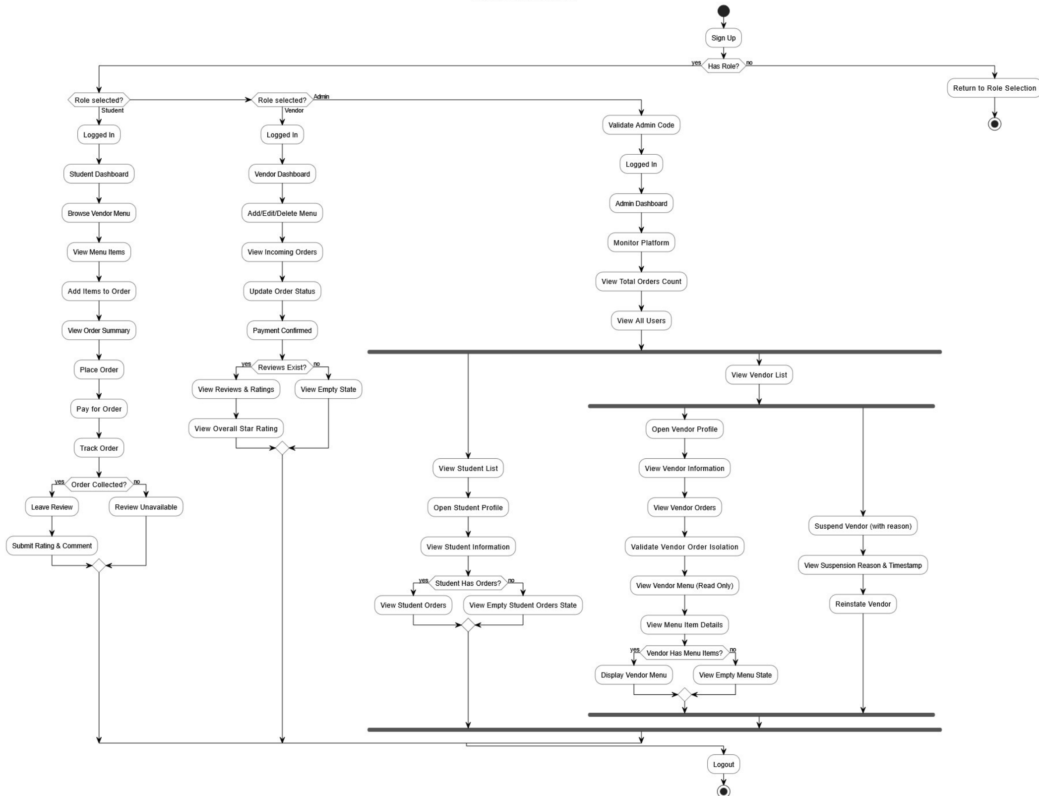
KuduDash Activity Diagram
