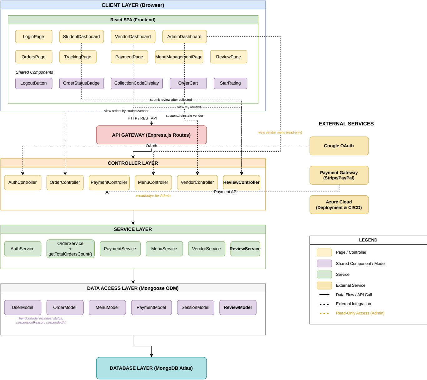
KUDUDASH - DEVELOPMENT VIEW (Component Diagram - Sprint 3)
